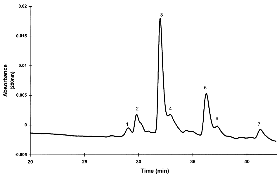
Fig. 3. HILIC chromatogram for the tryptic glycopeptides of Asn 25 from recombinant human interferon- \gamma following 120 h of a CHO cell batch culture.
