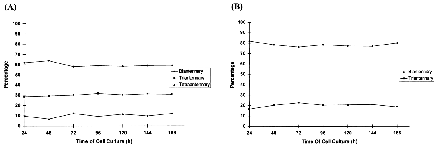
Fig. 5. (A) Antennarity percentages for the glycans of Asn 25 of IFN- \gamma during a suspension-batch CHO cell culture. (B) Antennarity percentages for the glycans of Asn 97 of IFN- \gamma during a suspension batch CHO cell culture.
